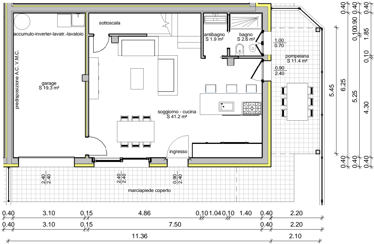
Piano terra
