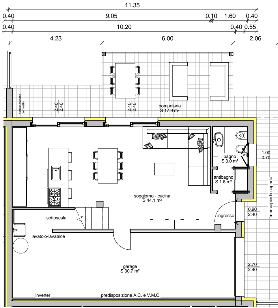
Piano terra Scala 1 : 100
