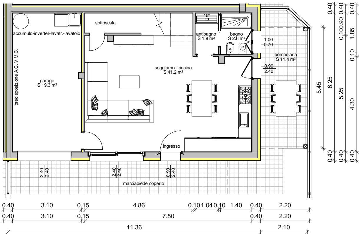
Piano terra
